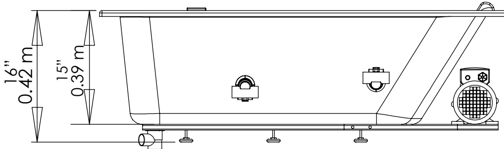
VISTA LATERAL / LATERAL VIEW
