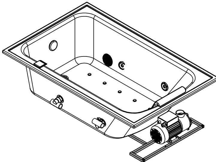
VISTA ISOMETRICO / ISOMETRIC VIEW
